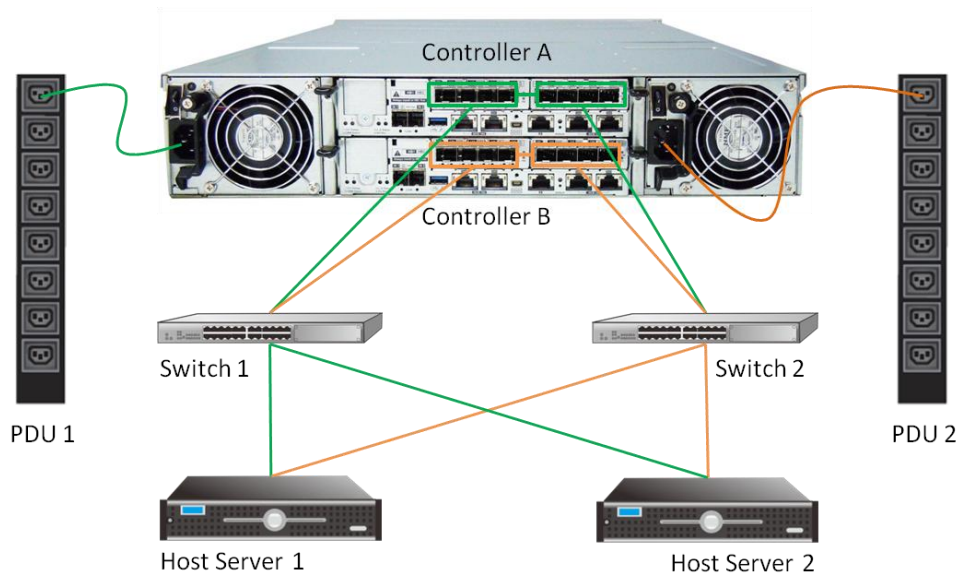
Block-Level HA Configuration
