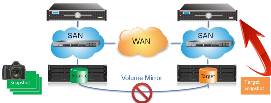
Disaster Recovery with Infortrend Remote Replication
