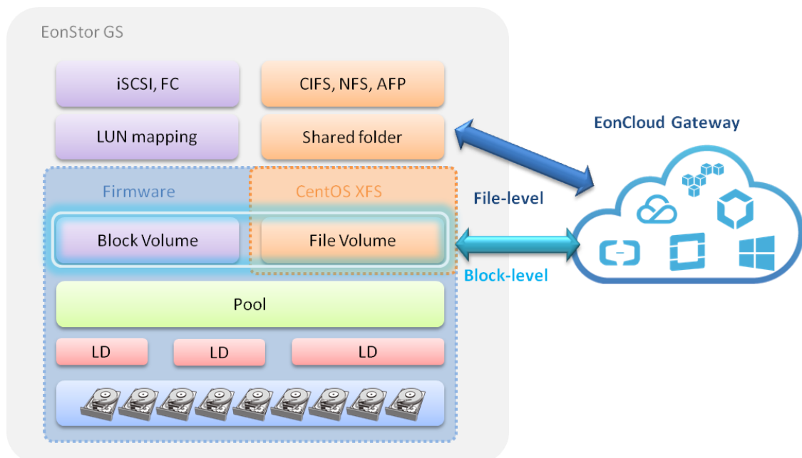
EonStor GS architecture
